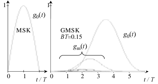
Figure 1: Pseudo-pulses for MSK ( BT=\infty ) and GMSK ( BT=0.15 ).
