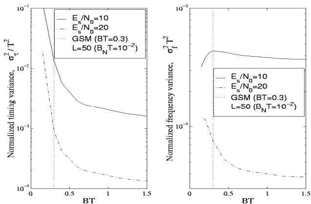
Figure 5: Impact of GMSK normalized Gaussian filter bandwidth, BT , on the UCRB (MSK corresponds to BT = \infty ).
