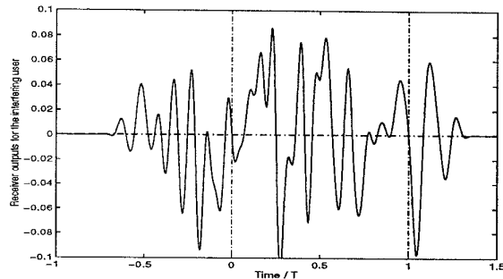
Figure 1: Conventional receiver one output vs. time
