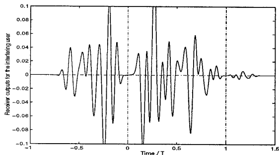
Figure 2: Robust receiver one output vs. time
