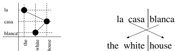
Fig. 1. Word and accent group alignment.
