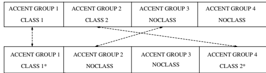
Fig. 4. Example of accent group alignment and class assignment.
